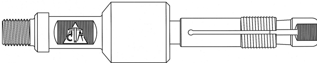
OPTION 1: 5/8 ROD PIN W/ 1 3/8 FISING NECK
